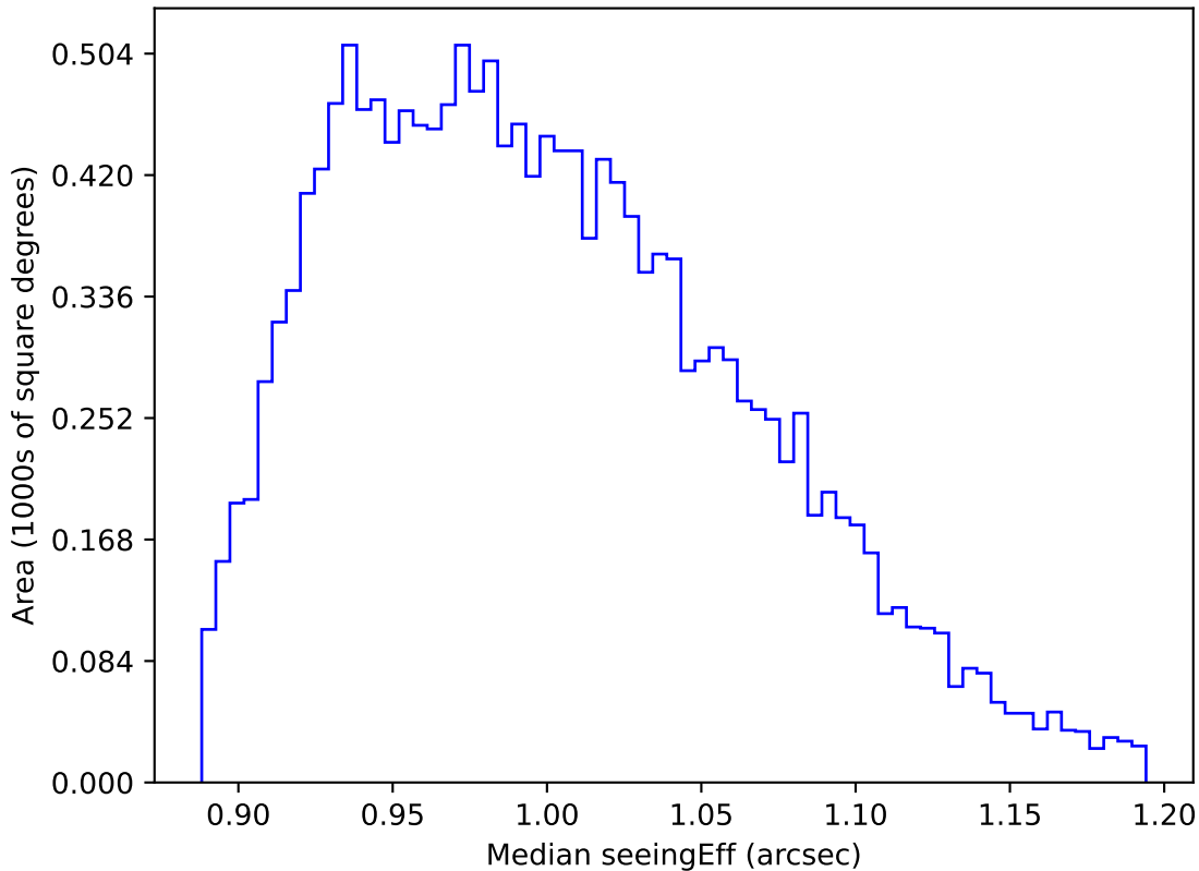
internal_u_expt38_nscale1.2v3.4_10yrs WFD y band: Median seeingEff
