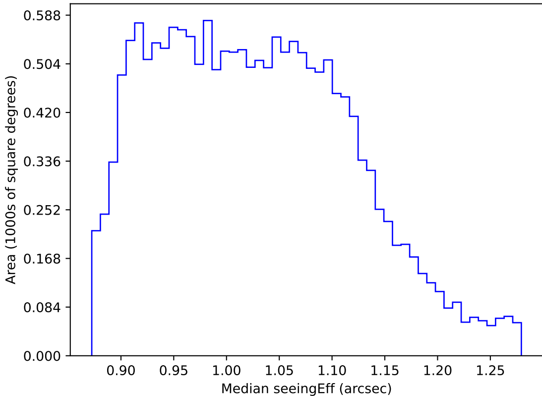
internal_u_expt38_nscale1.2v3.4_10yrs WFD r band: Median seeingEff
