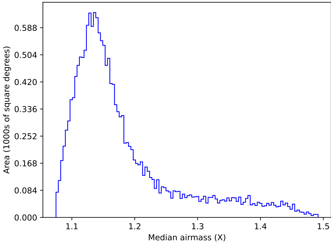
internal_u_expt38_nscale1.2v3.4_10yrs WFD g band: Median airmass
