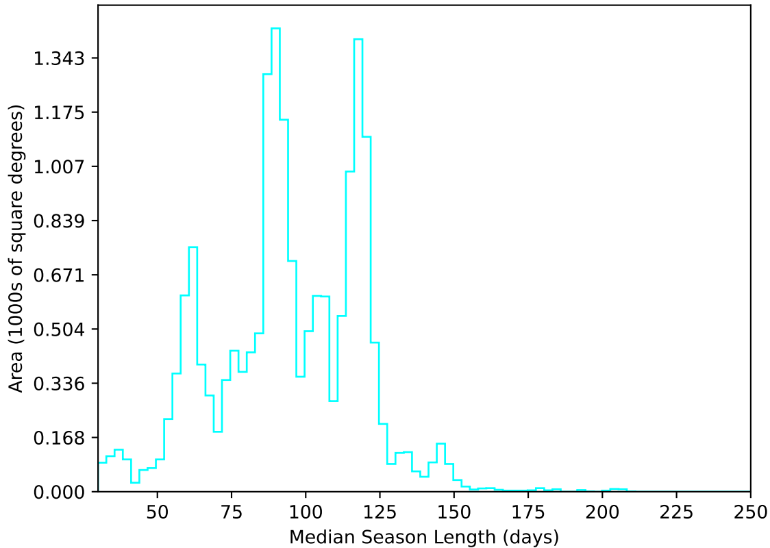
internal_u_expt38_nscale1.2v3.4_10yrs WFD u band: Median Season Length
