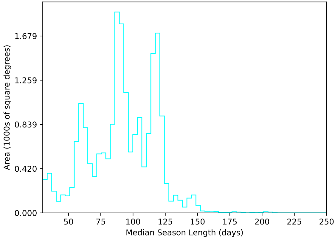
internal_u_expt38_nscale1.2v3.4_10yrs All sky u band: Median Season Length
