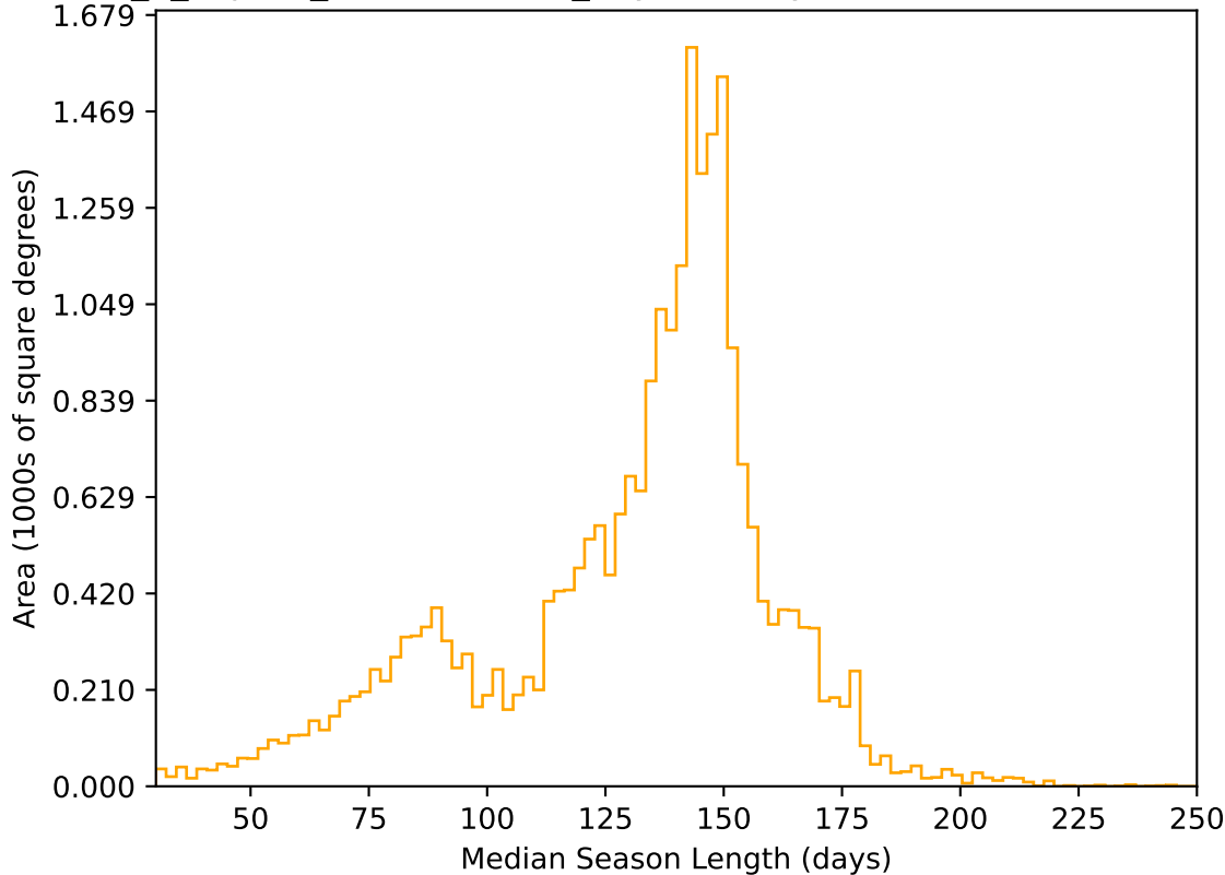
internal_u_expt38_nscale1.2v3.4_10yrs All sky r band: Median Season Length
