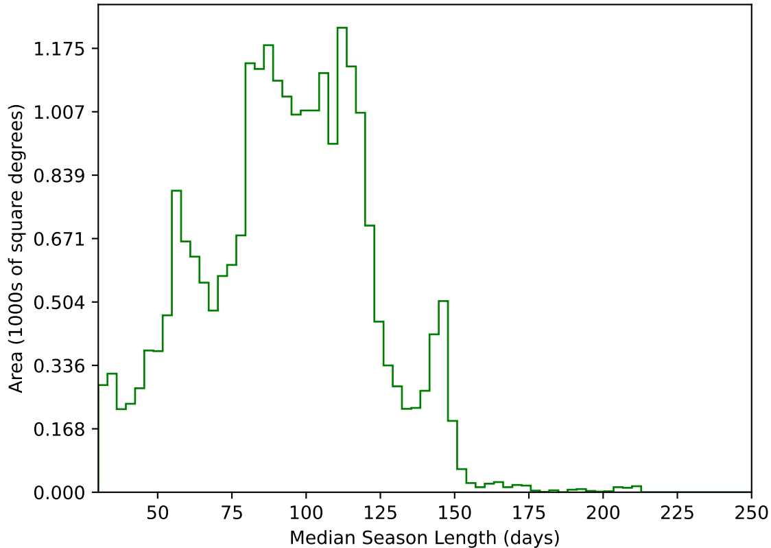
internal_u_expt38_nscale1.2v3.4_10yrs All sky g band: Median Season Length
