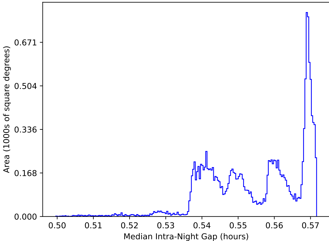
internal_u_expt38_nscale1.2v3.4_10yrs WFD: Median Intra-Night Gap
