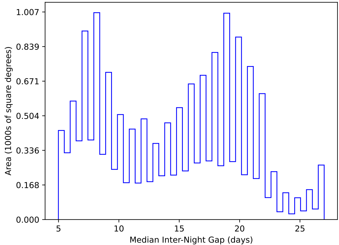
internal_u_expt38_nscale1.2v3.4_10yrs WFD y band: Median Inter-Night Gap
