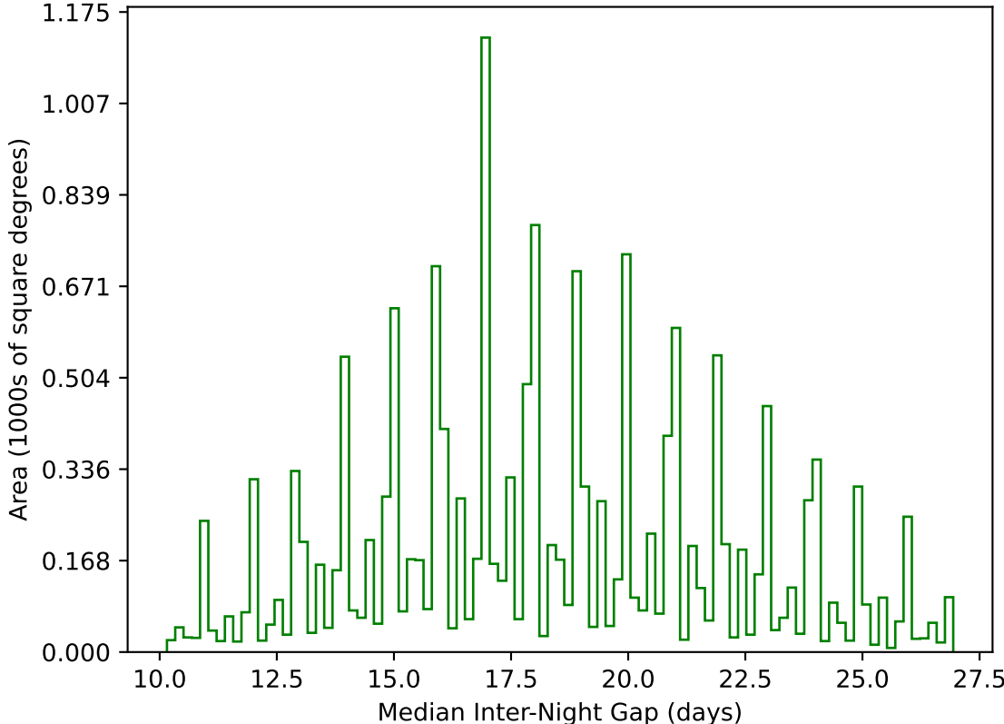
internal_u_expt38_nscale1.2v3.4_10yrs WFD g band: Median Inter-Night Gap
