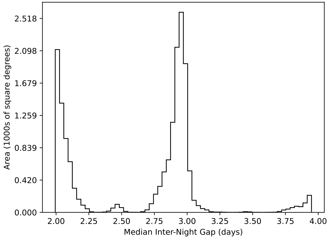
internal_u_expt38_nscale1.2v3.4_10yrs WFD all bands: Median Inter-Night Gap
