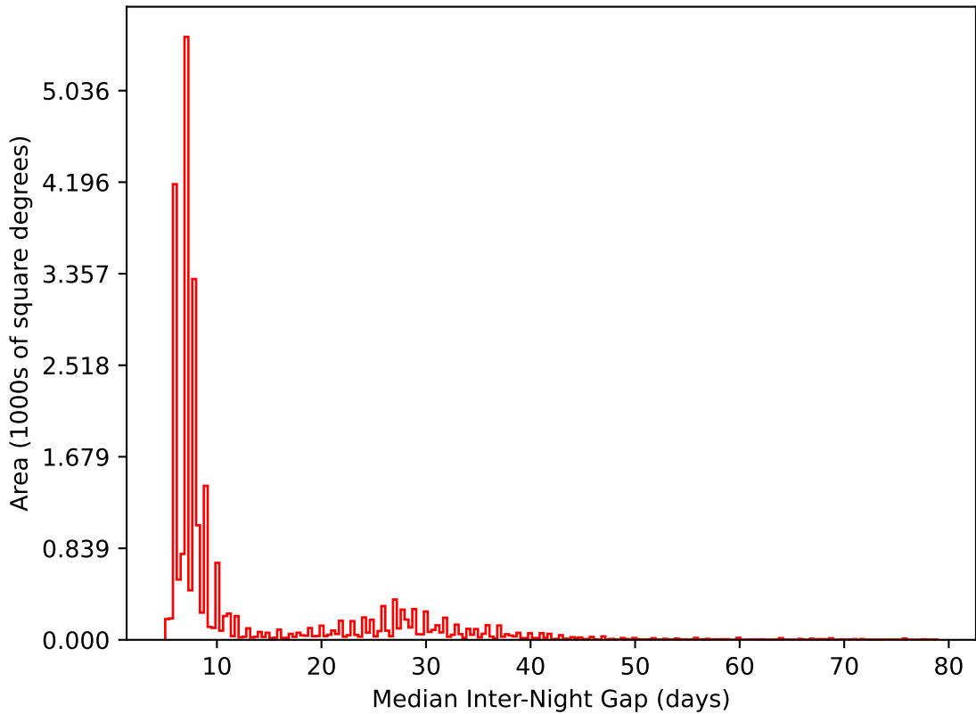
internal_u_expt38_nscale1.2v3.4_10yrs All sky i band: Median Inter-Night Gap
