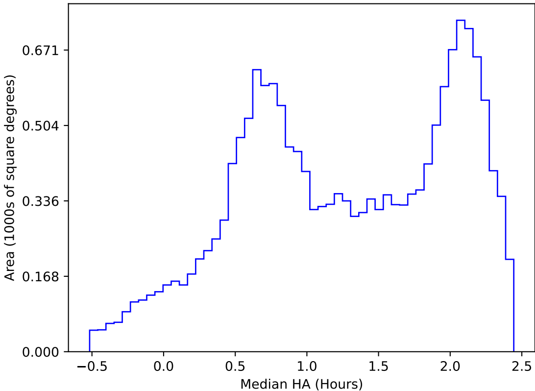
internal_u_expt38_nscale1.2v3.4_10yrs WFD y band: Median HA
