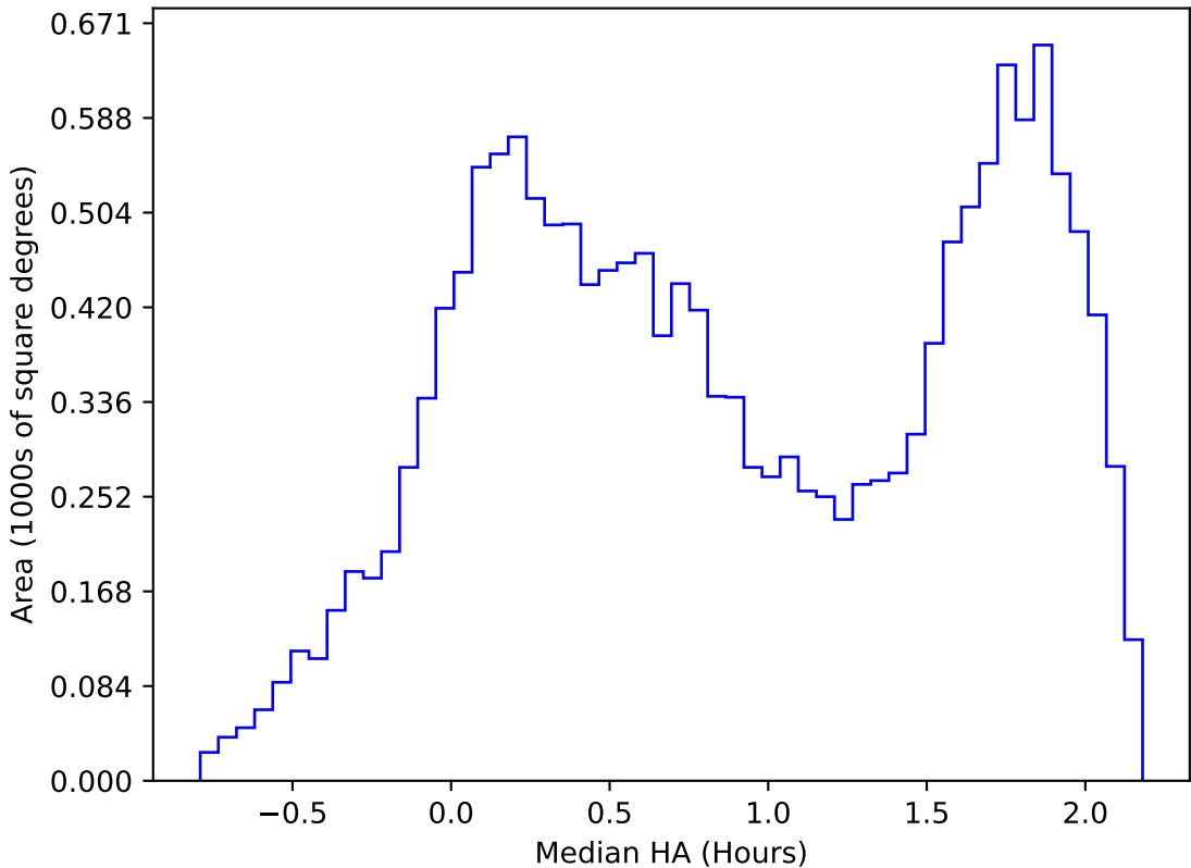
internal_u_expt38_nscale1.2v3.4_10yrs WFD r band: Median HA
