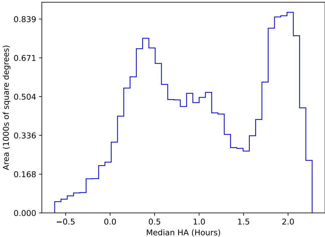
internal_u_expt38_nscale1.2v3.4_10yrs WFD i band: Median HA
