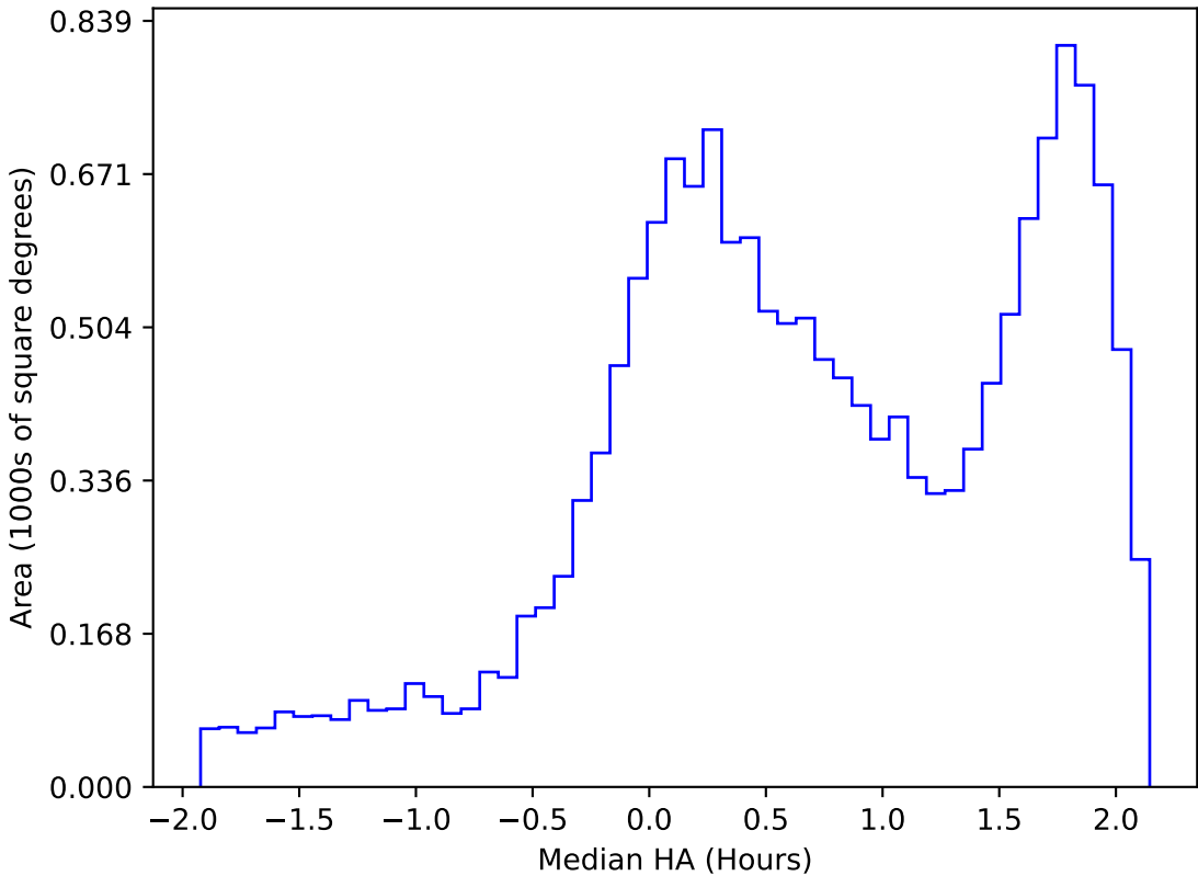
internal_u_expt38_nscale1.2v3.4_10yrs WFD g band: Median HA
