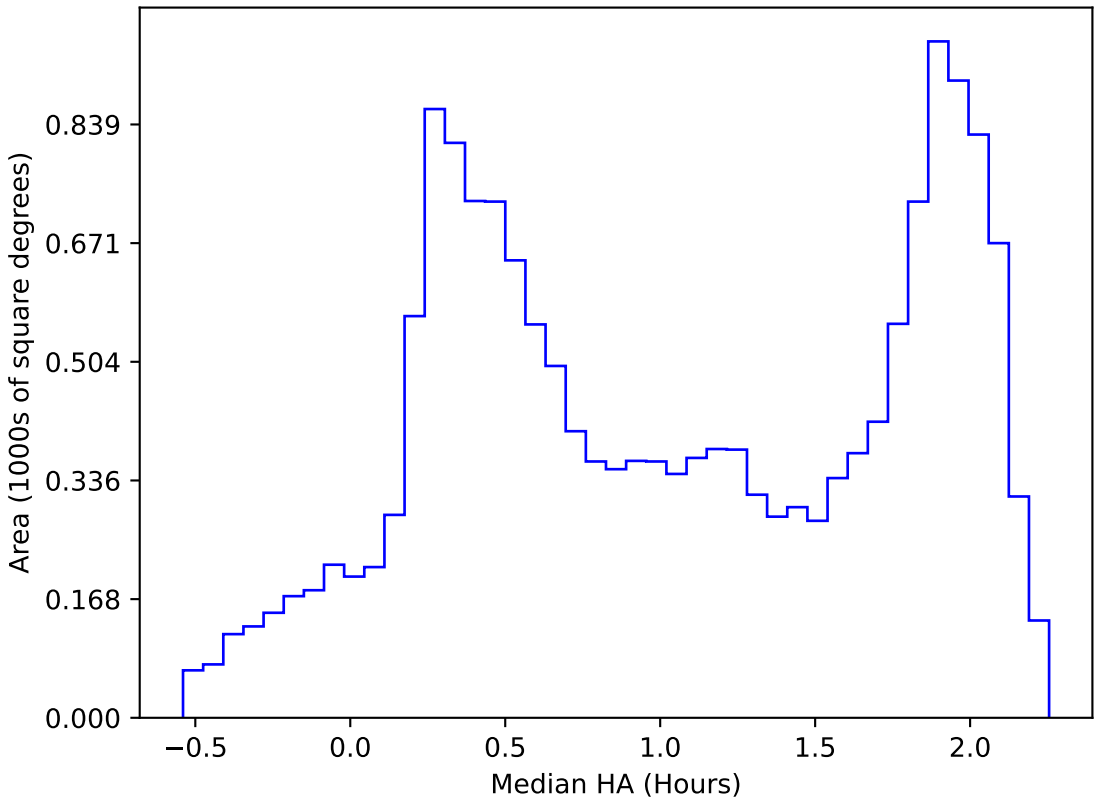
internal_u_expt38_nscale1.2v3.4_10yrs WFD all bands: Median HA
