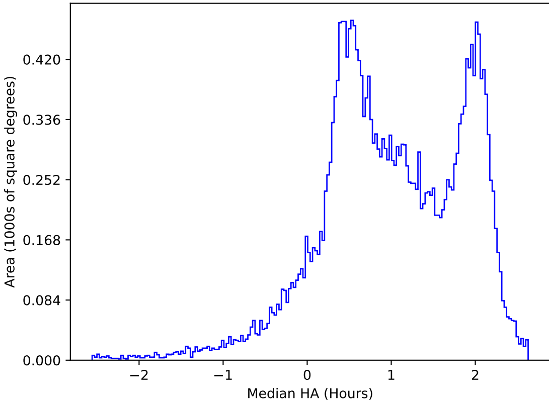
internal_u_expt38_nscale1.2v3.4_10yrs All sky z band: Median HA
