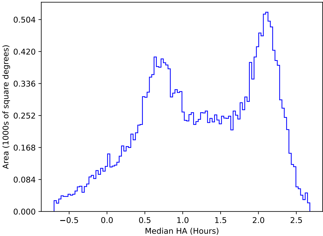
internal_u_expt38_nscale1.2v3.4_10yrs All sky y band: Median HA
