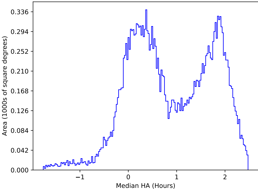
internal_u_expt38_nscale1.2v3.4_10yrs All sky u band: Median HA
