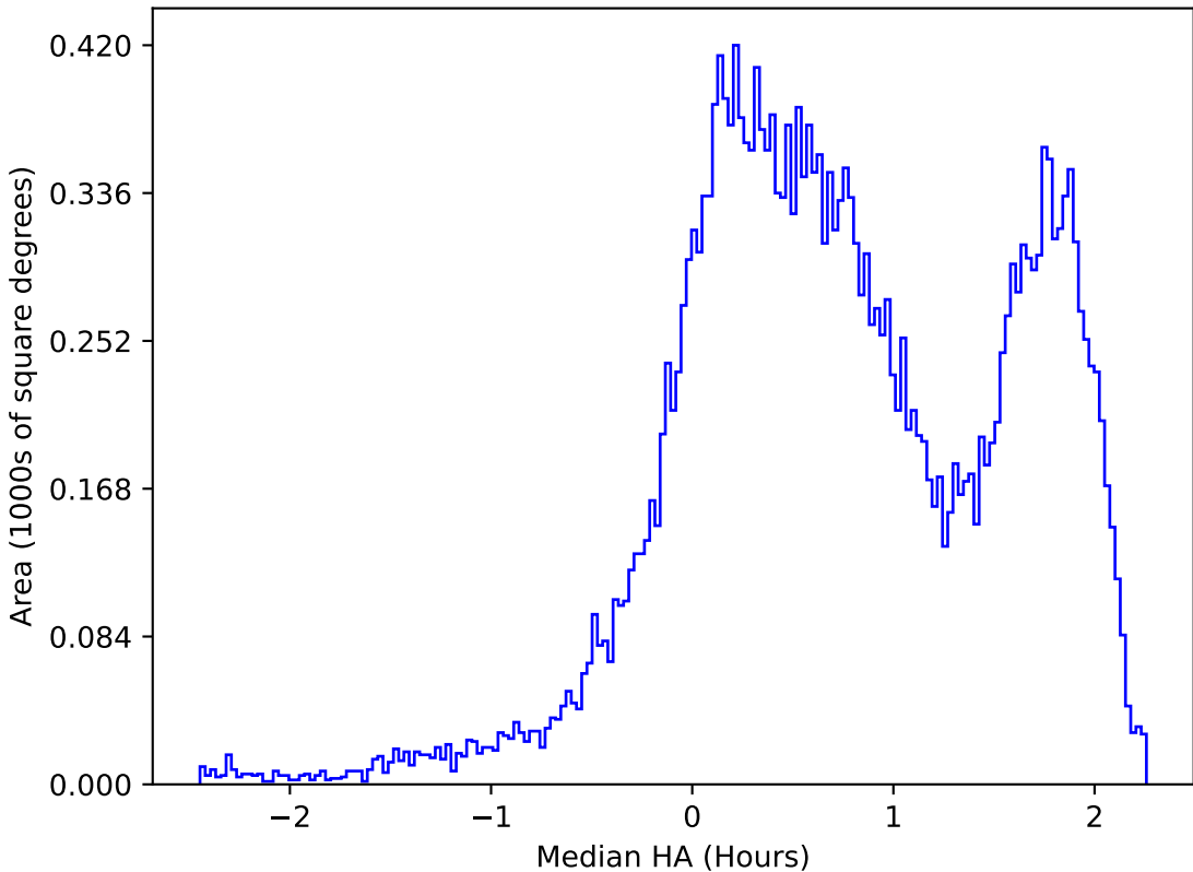
internal_u_expt38_nscale1.2v3.4_10yrs All sky r band: Median HA
