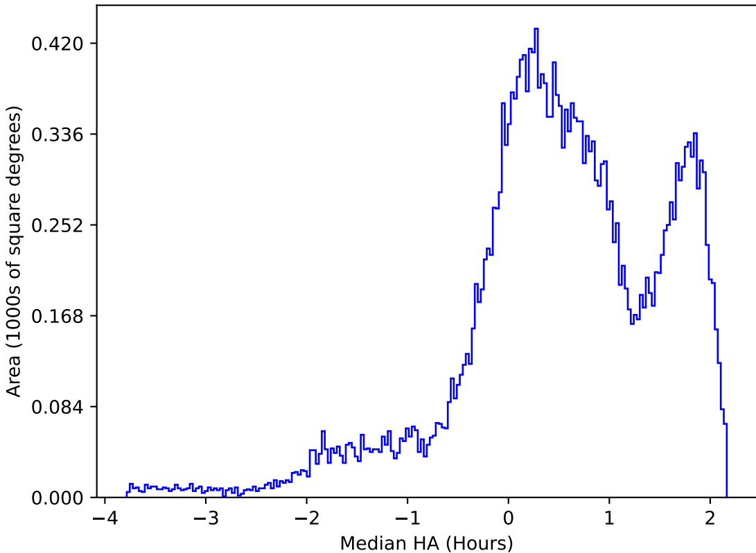
internal_u_expt38_nscale1.2v3.4_10yrs All sky g band: Median HA
