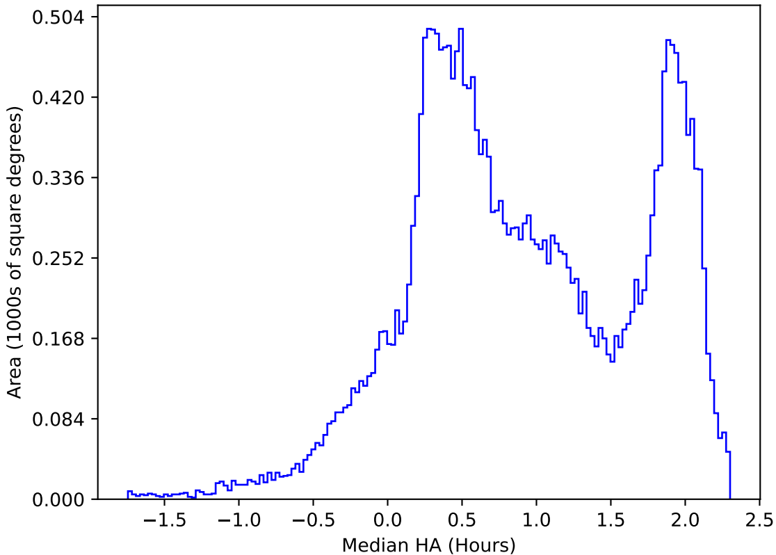
internal_u_expt38_nscale1.2v3.4_10yrs All sky all bands: Median HA
