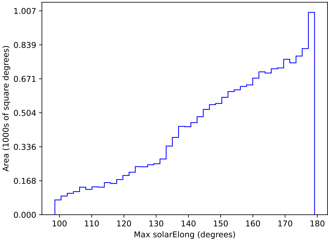
internal_u_expt38_nscale1.2v3.4_10yrs WFD y band: Max solarElong
