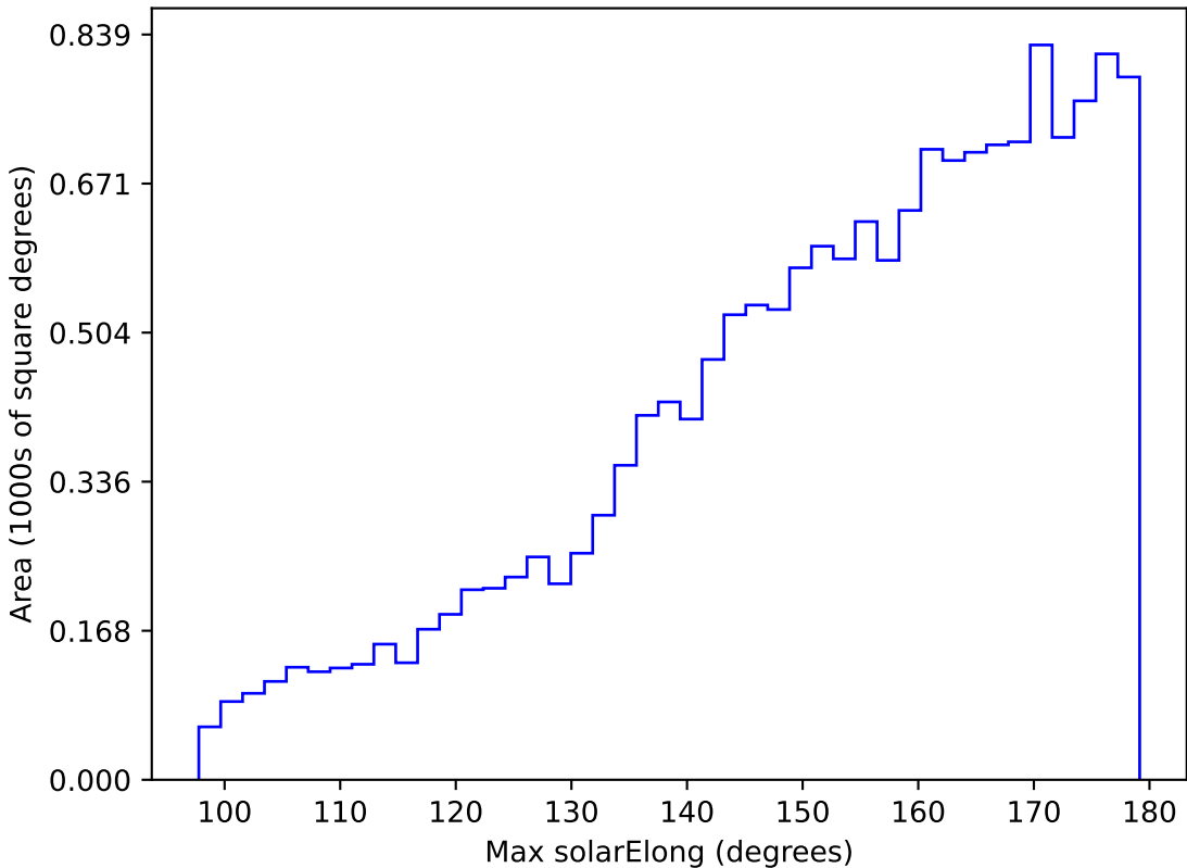
internal_u_expt38_nscale1.2v3.4_10yrs WFD u band: Max solarElong
