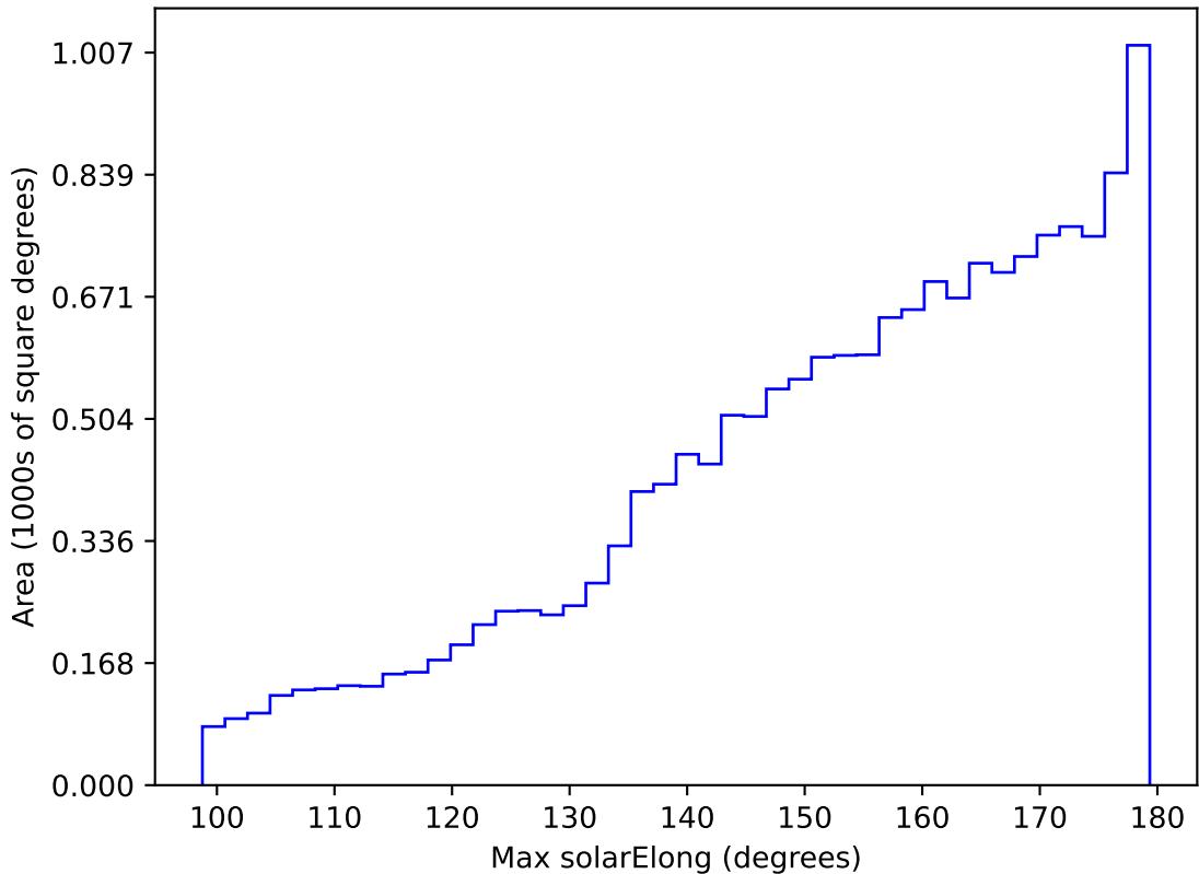
internal_u_expt38_nscale1.2v3.4_10yrs WFD r band: Max solarElong
