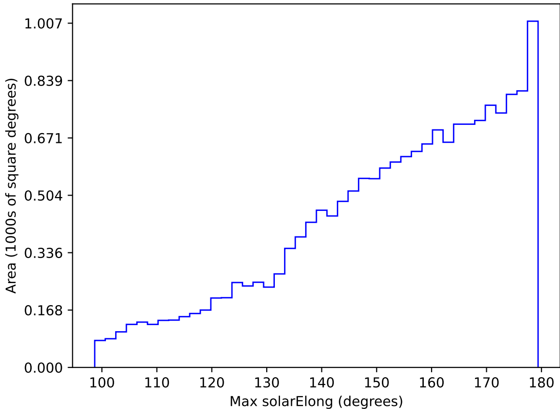
internal_u_expt38_nscale1.2v3.4_10yrs WFD i band: Max solarElong
