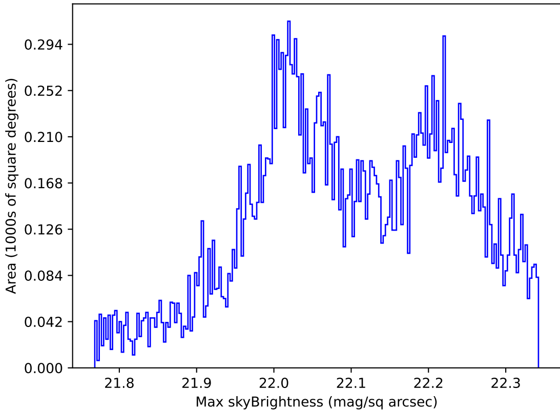
internal_u_expt38_nscale1.2v3.4_10yrs Yr 1 g band: Max skyBrightness
