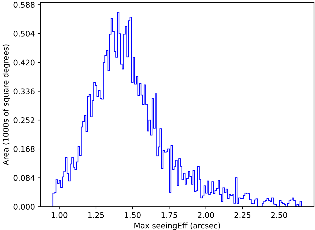
internal_u_expt38_nscale1.2v3.4_10yrs Yr 1 y band: Max seeingEff
