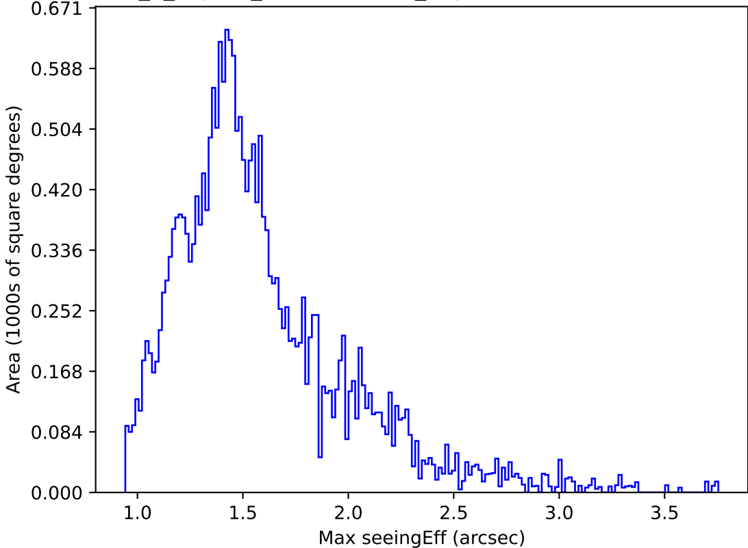
internal_u_expt38_nscale1.2v3.4_10yrs Yr 1 u band: Max seeingEff
