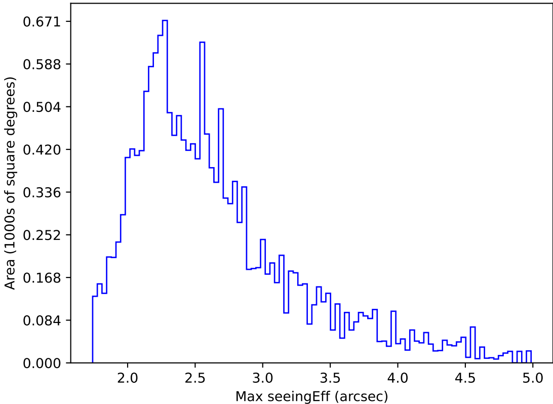
internal_u_expt38_nscale1.2v3.4_10yrs WFD z band: Max seeingEff
