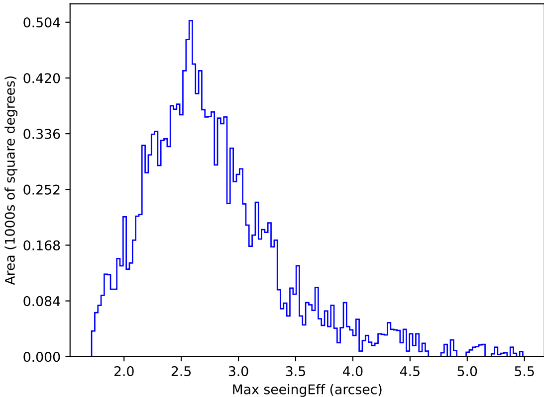
internal_u_expt38_nscale1.2v3.4_10yrs WFD r band: Max seeingEff
