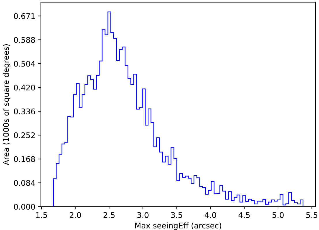
internal_u_expt38_nscale1.2v3.4_10yrs WFD i band: Max seeingEff
