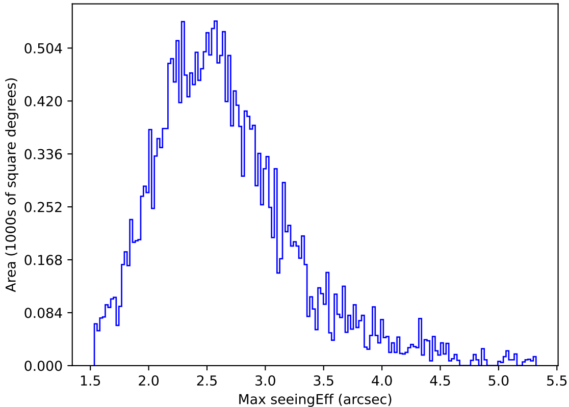
internal_u_expt38_nscale1.2v3.4_10yrs All sky r band: Max seeingEff
