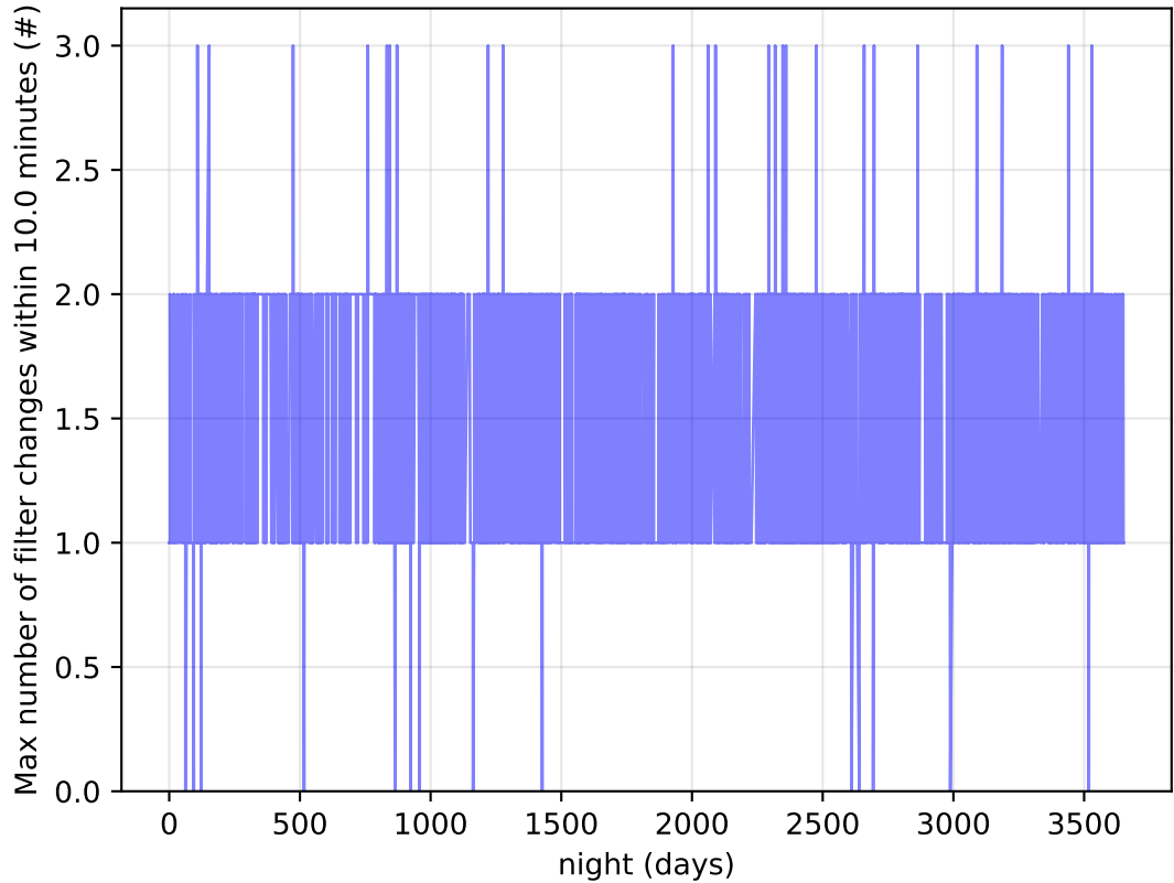
internal_u_expt38_nscale1.2v3.4_10yrs Per Night: Max number of filter changes within 10.0 minutes
