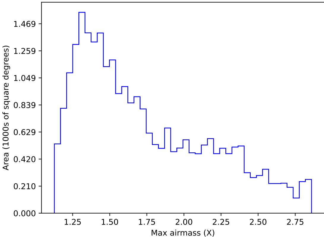
internal_u_expt38_nscale1.2v3.4_10yrs Yr 1 z band: Max airmass
