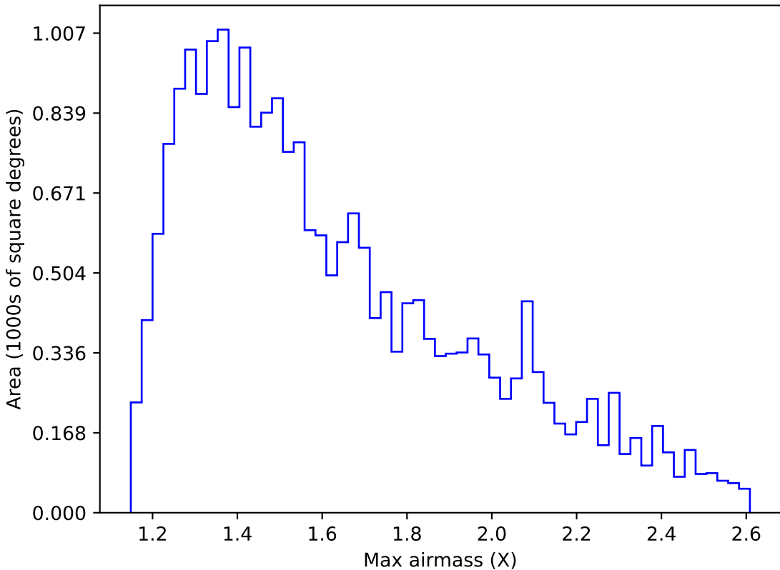
internal_u_expt38_nscale1.2v3.4_10yrs Yr 1 y band: Max airmass
