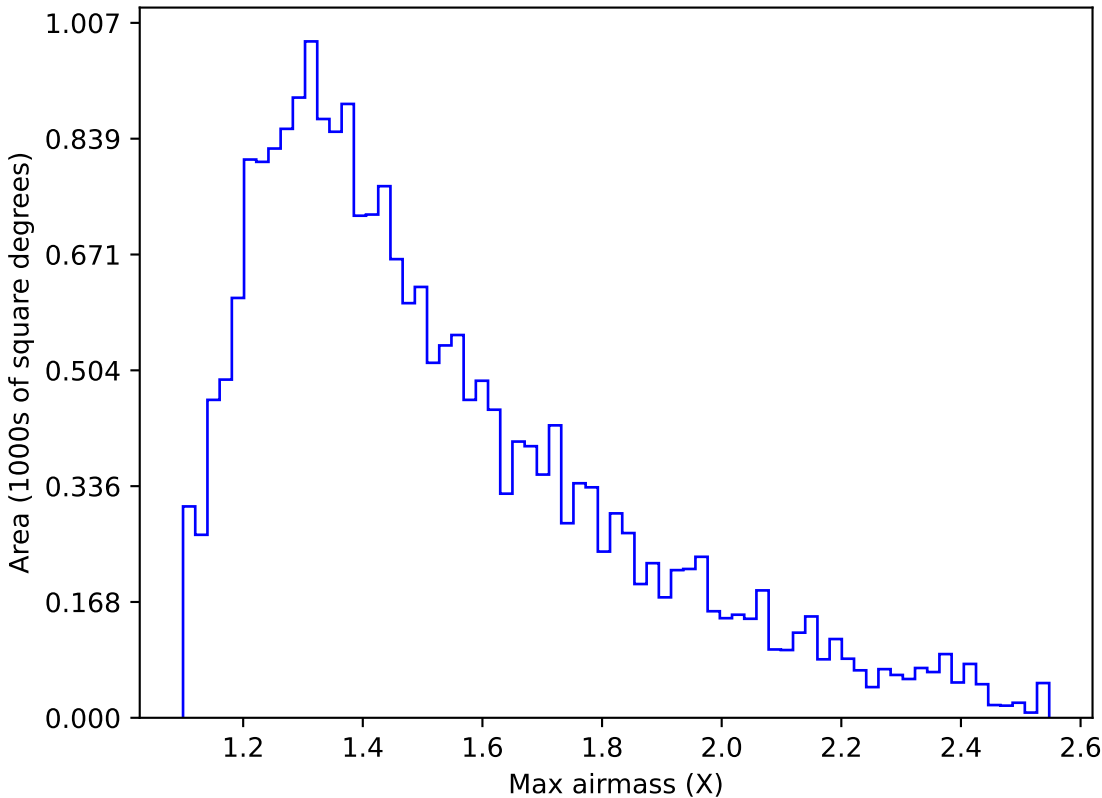
internal_u_expt38_nscale1.2v3.4_10yrs Yr 1 u band: Max airmass
