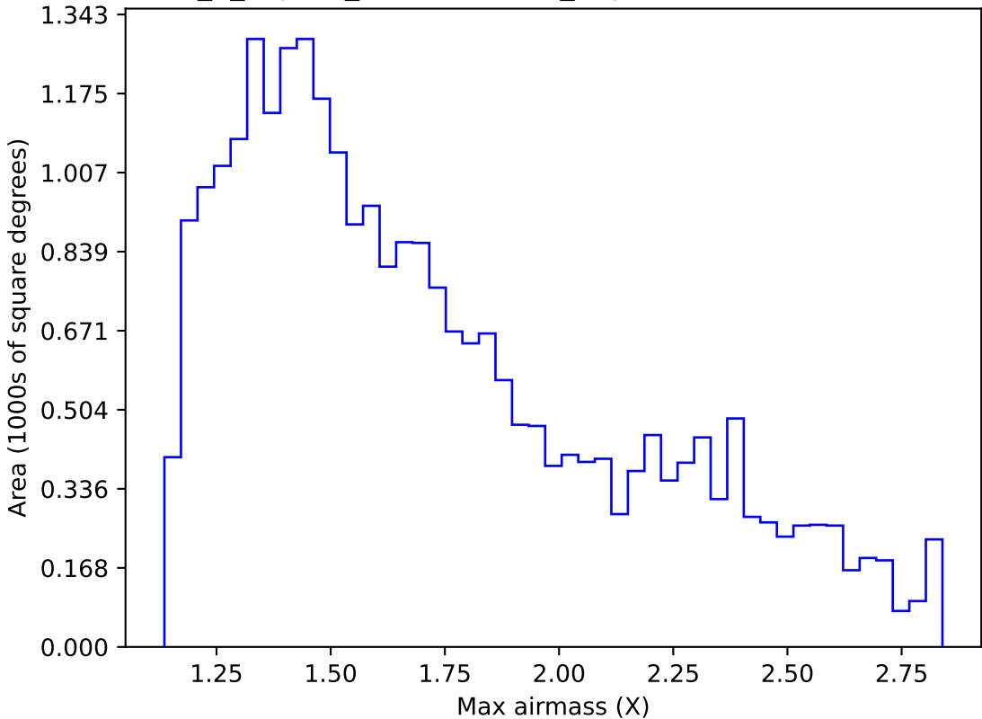
internal_u_expt38_nscale1.2v3.4_10yrs Yr 1 i band: Max airmass
