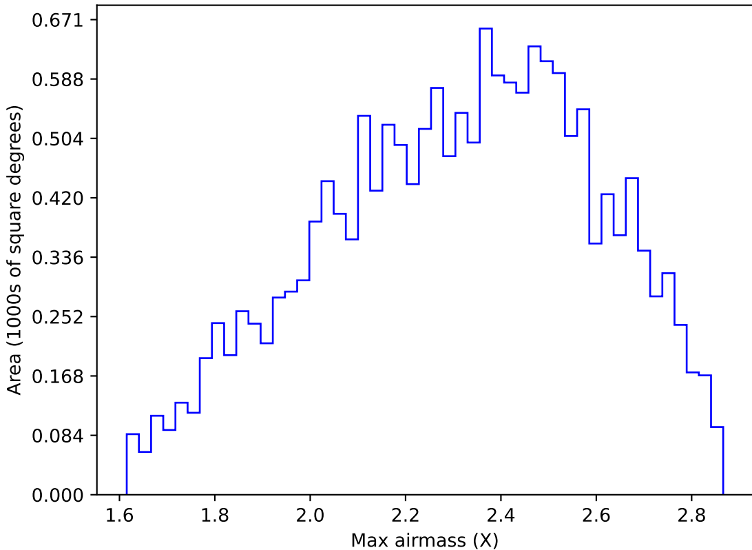
internal_u_expt38_nscale1.2v3.4_10yrs WFD y band: Max airmass
