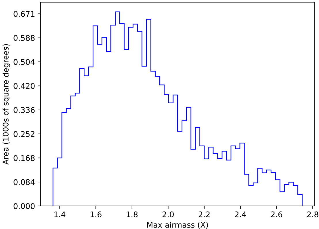
internal_u_expt38_nscale1.2v3.4_10yrs WFD u band: Max airmass
