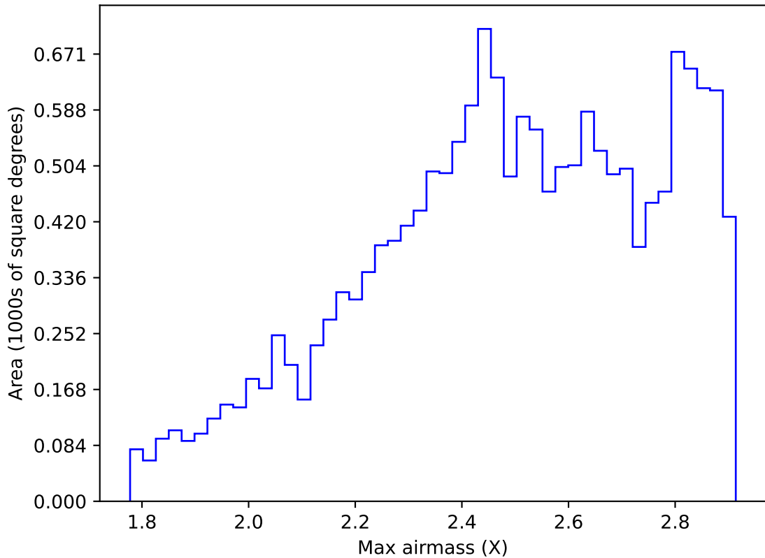
internal_u_expt38_nscale1.2v3.4_10yrs WFD i band: Max airmass
