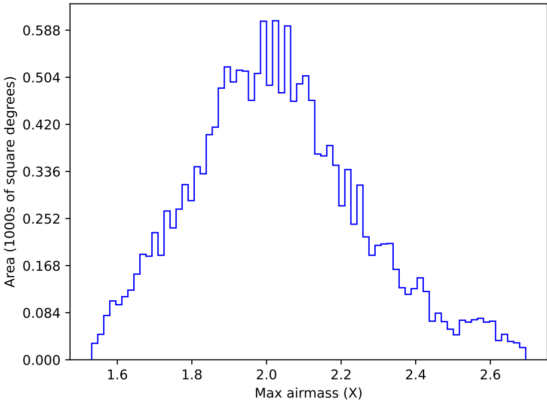
internal_u_expt38_nscale1.2v3.4_10yrs WFD g band: Max airmass
