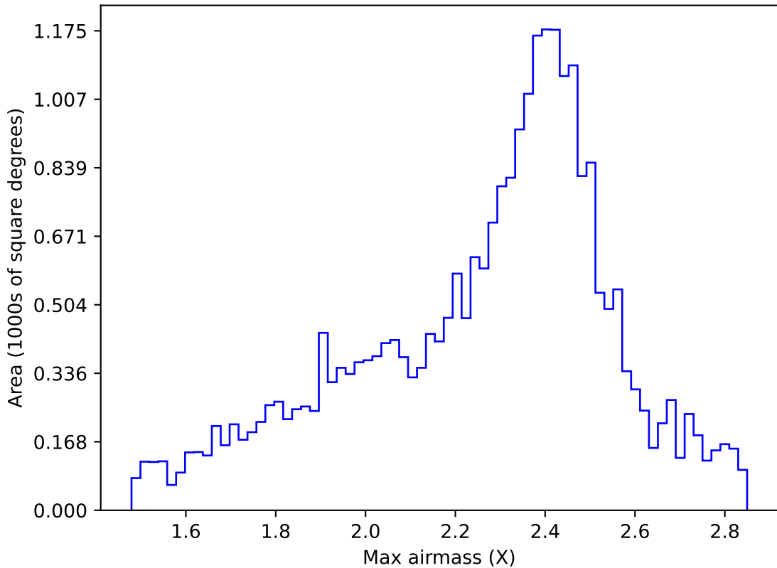
internal_u_expt38_nscale1.2v3.4_10yrs All sky r band: Max airmass
