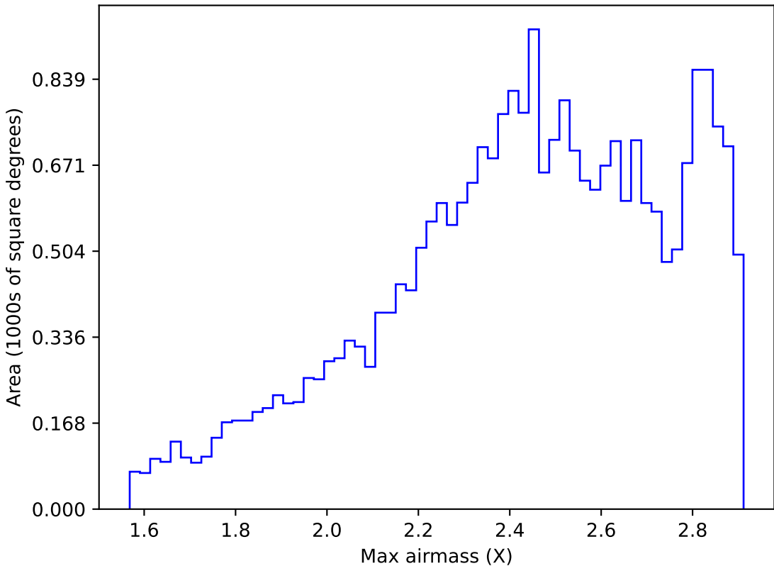
internal_u_expt38_nscale1.2v3.4_10yrs All sky i band: Max airmass
