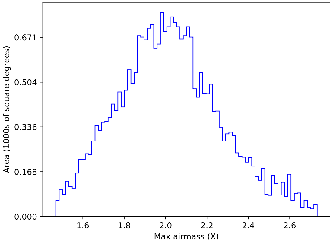
internal_u_expt38_nscale1.2v3.4_10yrs All sky g band: Max airmass
