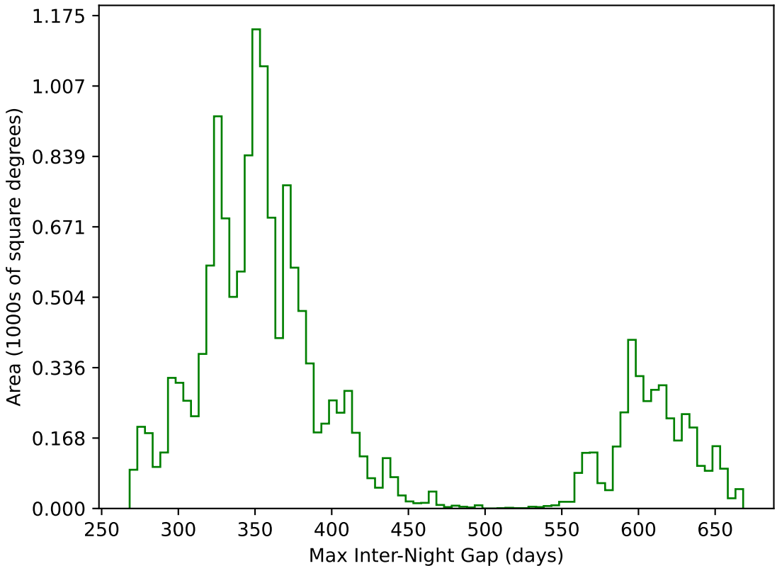
internal_u_expt38_nscale1.2v3.4_10yrs WFD g band: Max Inter-Night Gap
