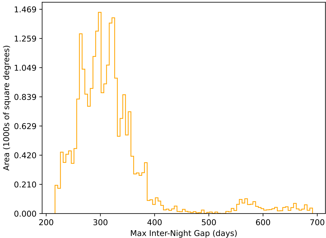
internal_u_expt38_nscale1.2v3.4_10yrs All sky r band: Max Inter-Night Gap
