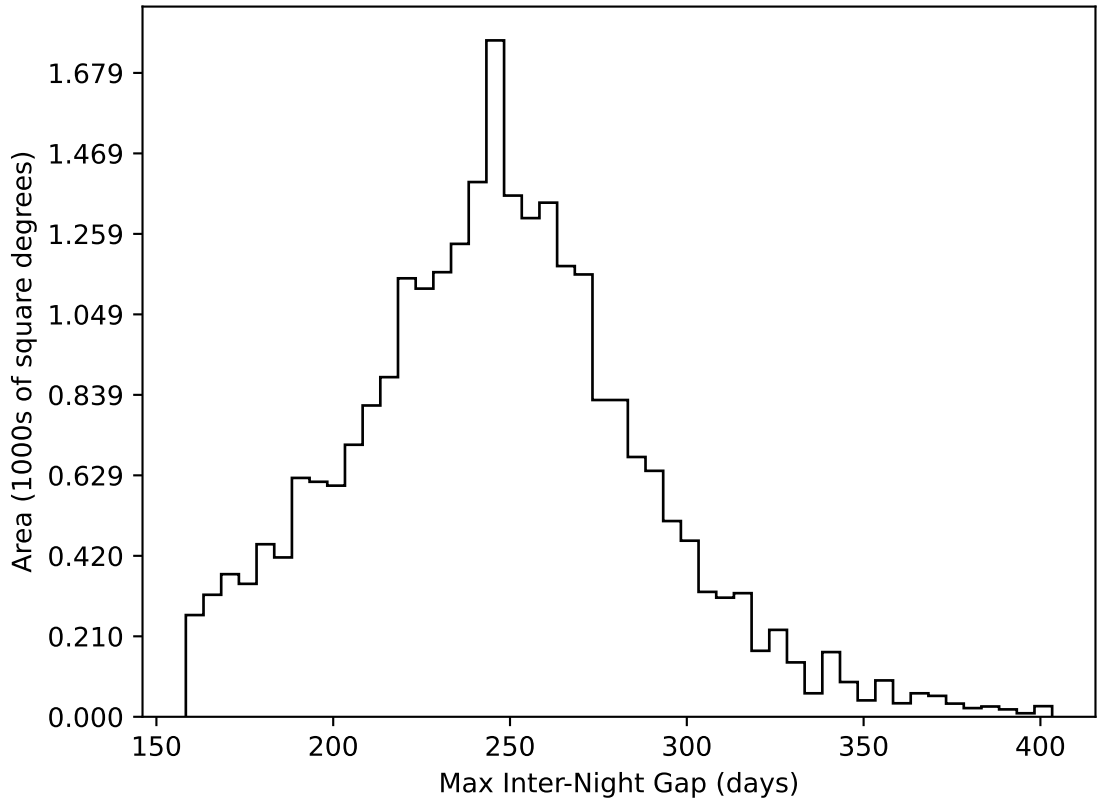
internal_u_expt38_nscale1.2v3.4_10yrs All sky all bands: Max Inter-Night Gap
