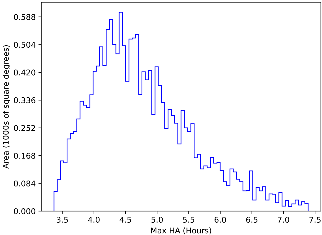
internal_u_expt38_nscale1.2v3.4_10yrs WFD y band: Max HA
